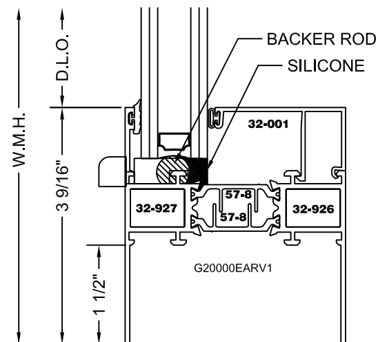
FX/PI FRAME (1-1/2" EXT)
