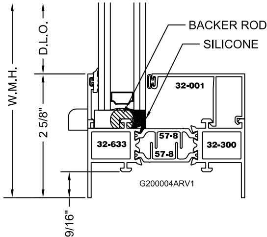
FX/PI FEMALE STACK FRAME
