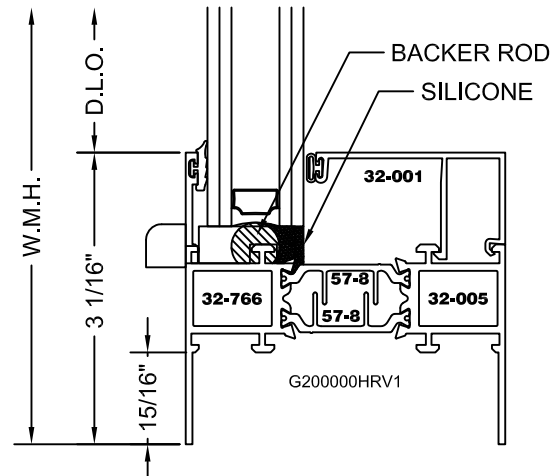
FX/PI (EX) FRAME
