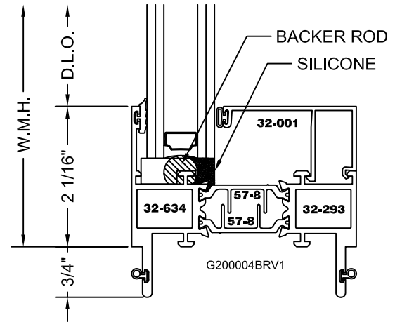
FX/PI MALE STACK FRAME
