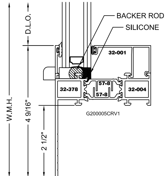
FX/PI (2-1/2\" EX-EXT/UN-EQ) LEG FRAME
