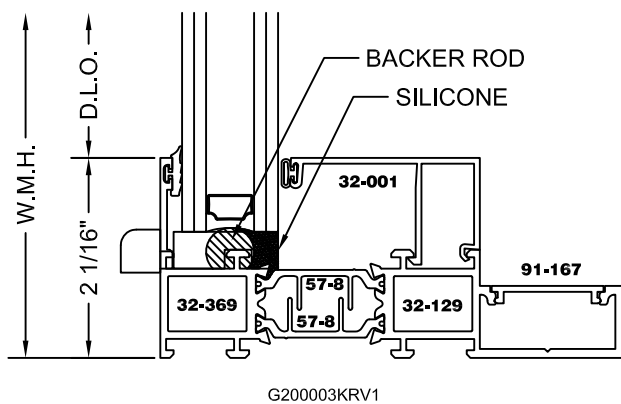
FX/PI BLAST TRIM W/POCKET
