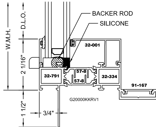
FX/PI BLAST TRIM OFFSET POCKET (EXT-NF)
