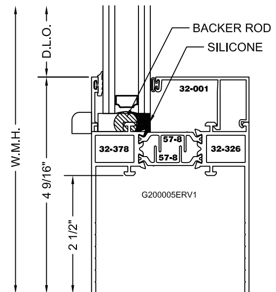
FX/PI (2-1/2" EXT) FRAME
