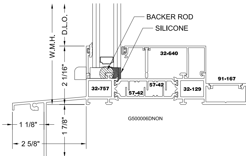
FX/PI FRAME (STUCCO-PAN) W/ TRIM POCKET
