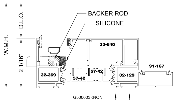
FX/PI BLAST TRIM W/POCKET
