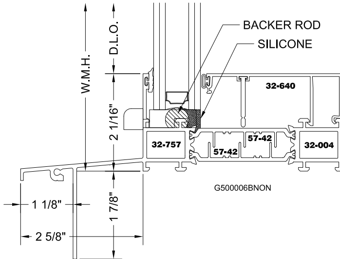
FX/PI FRAME (STUCCO-PAN) (HINGE OFFSET)
