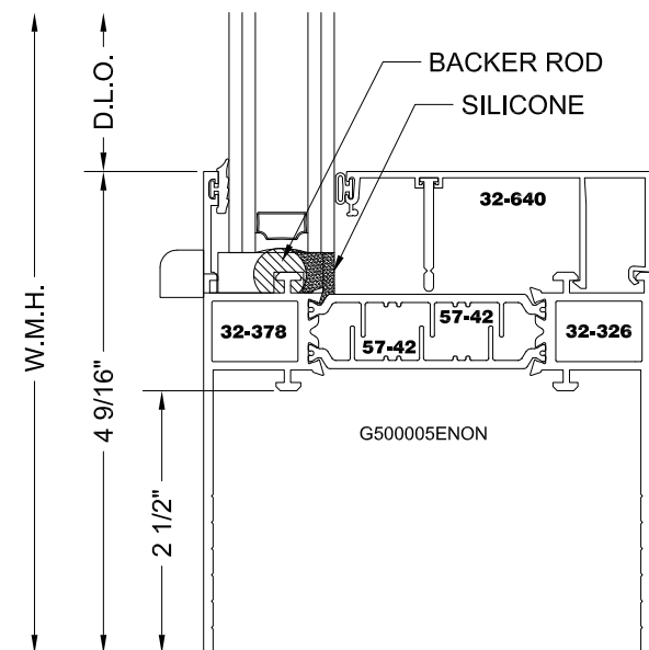
FX/PI (2-1/2\" EXT) FRAME
