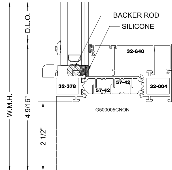
FX/PI (2-1/2" EX-EXT/UN-EQ) LEG FRAME
