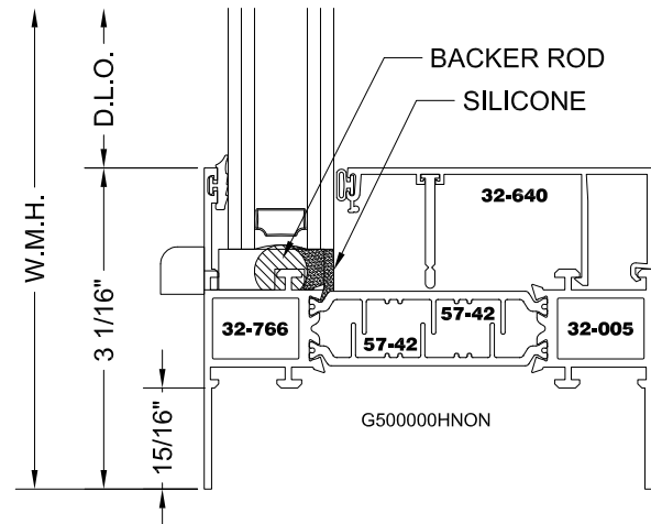
FX/PI (EX) FRAME
