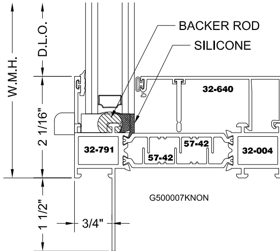
FX/PI BLAST TRIM W/POCKET
