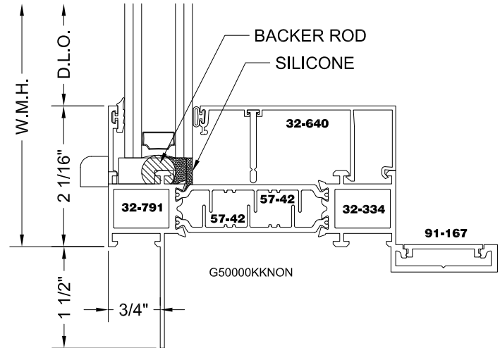
FX/PI BLAST TRIM OFFSET POCKET (EXT-NF)
