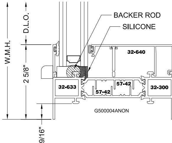
FX/PI FEMALE STACK FRAME
