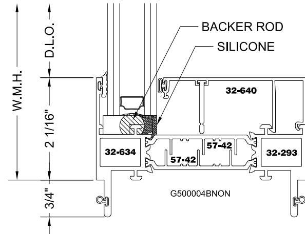
FX/PI MALE STACK FRAME
