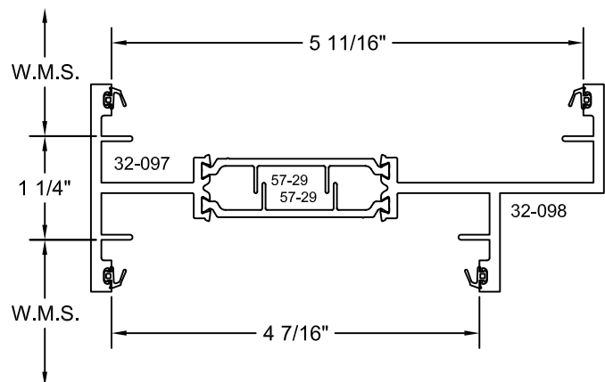
G5ME
