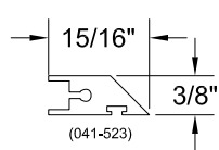
APPLIED GRID FRAME (HISTORIC G600 GRID FRAME)
