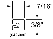
APPLIED GRID FRAME (STANDARD G600 GRID FRAME)
