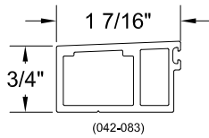
APPLIED GRID FRAME (LARGE OFFSET GRID FRAME)
