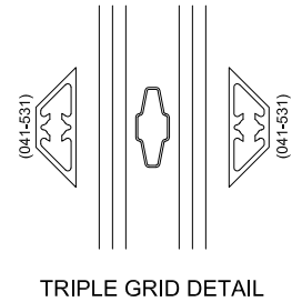
TRIPLE GRID DETAIL
