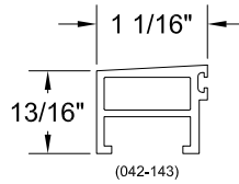
APPLIED GRID FRAME (OFFSET GRID FRAME - G600 CORNER KEY)
