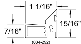
APPLIED GRID FRAME (G600 OFFSET GRID FRAME - PUTTY)
