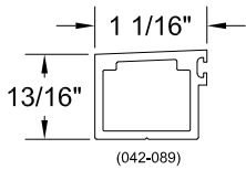
APPLIED GRID FRAME (STANDARD OFFSET GRID FRAME)
